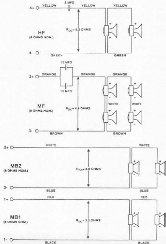
FIGURE 7 — MTH-4.5/64B Wiring Diagram
